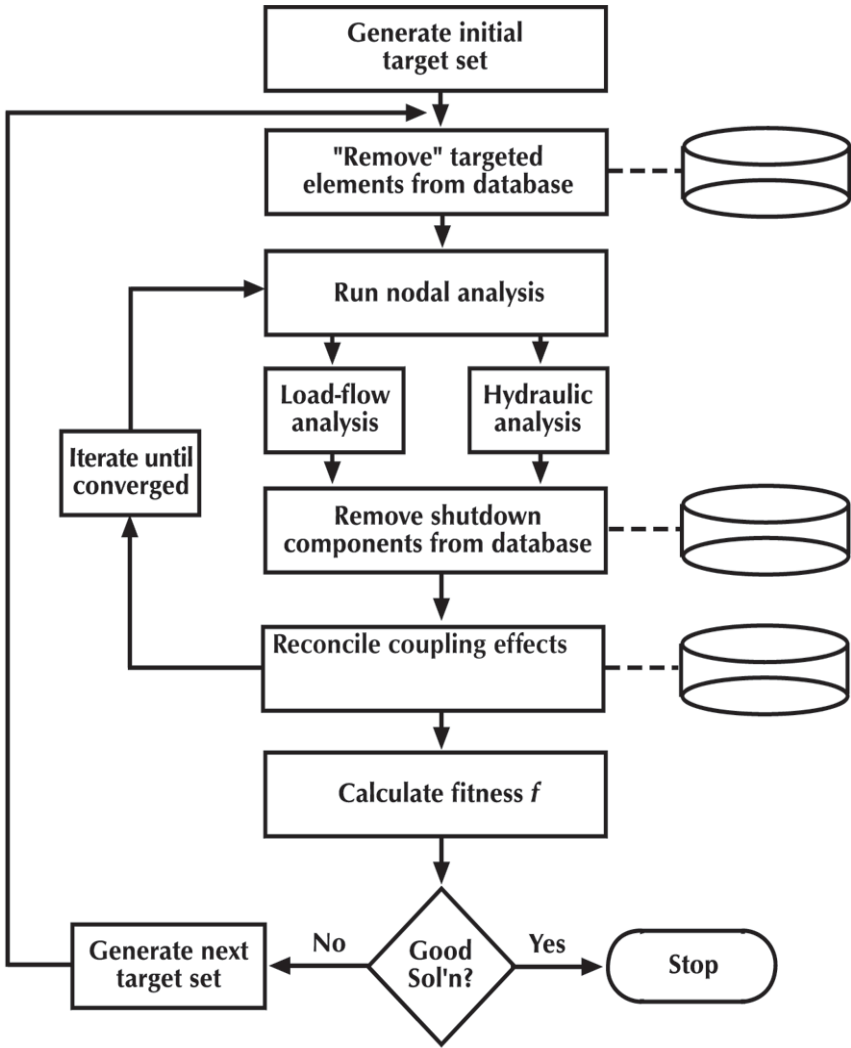
Figure 8.1: Genetic Algorithm Flow
