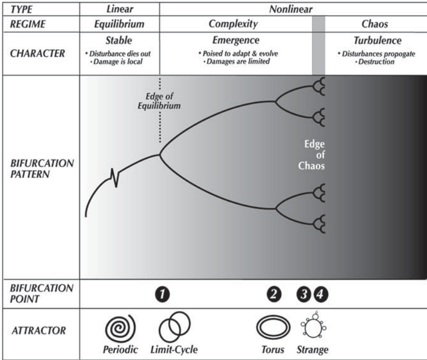
Figure 3.1: Period-Doubling Cascade
